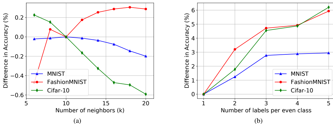
Figure 2. Accuracy of Poisson Learning for (a) different numbers of neighbors k used to construct the graph and (b) unbalanced training data. In (a) we used 5 labels per class and in (b) we used 1 label per class for the odd numbered classes, and m = 1, 2, 3, 4, 5 labels per class for the even numbered classes. Both figures show the difference in accuracy compared to k = 10 and balanced training data.
