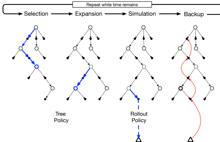
Figure 8.11: Monte Carlo Tree Search. When the environment changes to a new state, MCTS executes as many iterations as possible before an action needs to be selected, incrementally building a tree whose root node represents the current state. Each iteration consists of the four operations Selection , Expansion (though possibly skipped on some iterations), Simulation , and Backup , as explained in the text and illustrated by the bold arrows in the trees. Adapted from Chaslot, Bakkes, Szita, and Spronck (2008).
