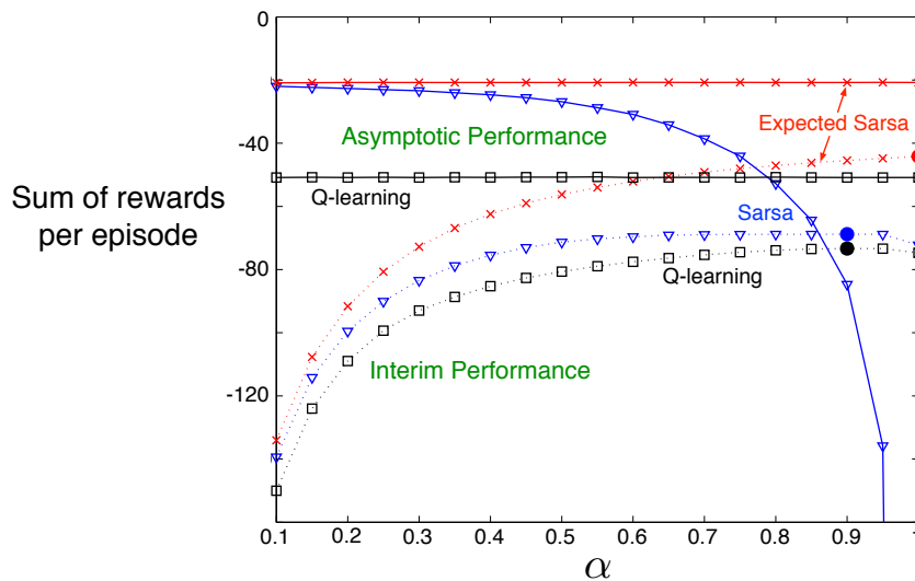
Figure 6.6: Interim and asymptotic performance of TD control methods on the cliff-walking task as a function of \alpha . All algorithms used an \epsilon -greedy policy with \epsilon = 0.1 . Asymptotic performance is an average over 100,000 episodes whereas interim performance is an average over the first 100 episodes. These data are averages of over 50,000 and 10 runs for the interim and asymptotic cases respectively. The solid circles mark the best interim performance of each method. Adapted from van Seijen et al. (2009).
