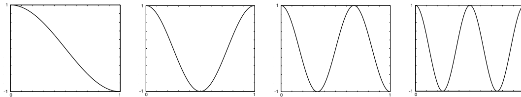
Figure 9.3: One-dimensional Fourier cosine-basis features x_i , i = 1, 2, 3, 4 , for approximating functions over the interval [0, 1] . After Konidaris et al. (2011).
