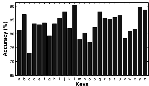
Figure 7: Mean accuracy for keys A-Z (Users 1-10)
