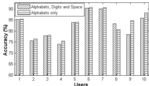
Figure 9: Per user average classifier accuracies
