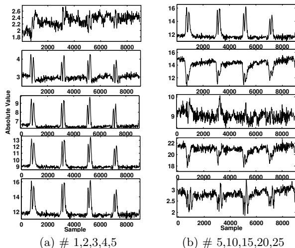
Figure 3: Correlated variations in subcarriers
