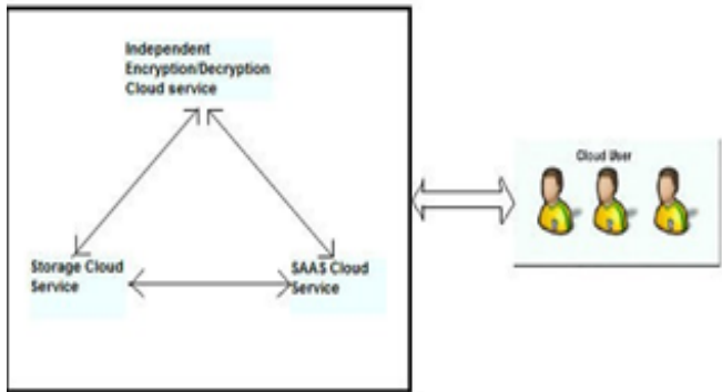
Fig3.Security Agreement framework integrating separate cloud services for data encryption/decryption, SAAS and storage
