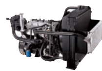
D4CB(A-ENG) 146ps/3,600rpm / 28kg.m/3,600rpm / 2,497cc
