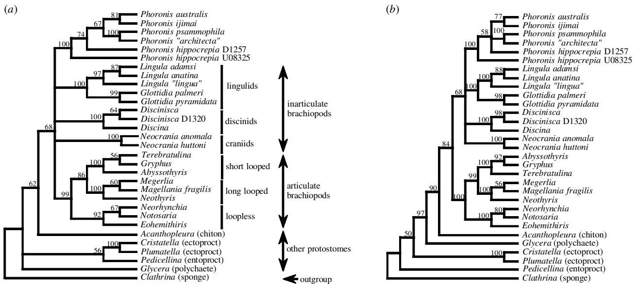
Figure 1. Phylogenetic analyses of 18S rDNA sequences. (a) Maximum parsimony bootstrap 50% consensus of 100 heuristic searches with ten random addition replicates and tree bisection–reconnection branch exchange, without steepest descent. Zero-length branches and nodes with less than 50% support were collapsed. Acctran optimization enforced. The single most parsimonious tree obtained under the same search conditions (288 informative sites) was 862 steps total length, CI = 0.52, RI = 0.69 (not shown). (b) Minimum evolution, neighbour-joining, bootstrap 50% consensus tree based on Kimura pairwise distances calculated from 1000 pseudoreplicates based on all substitutions, assuming no sites invariant, gap sites ignored, ties (if any) broken arbitrarily and negative branch lengths set to zero.
