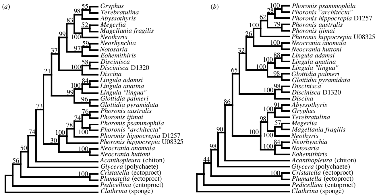
Figure 2. Phylogenetic analyses of 18S rDNA sequences. (a, b) As figure 1a,b except that nodes with less than 50% support were not collapsed.
