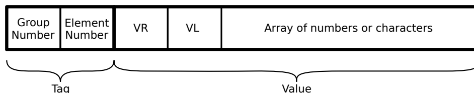
Figure 1: A DICOM DataElement.
