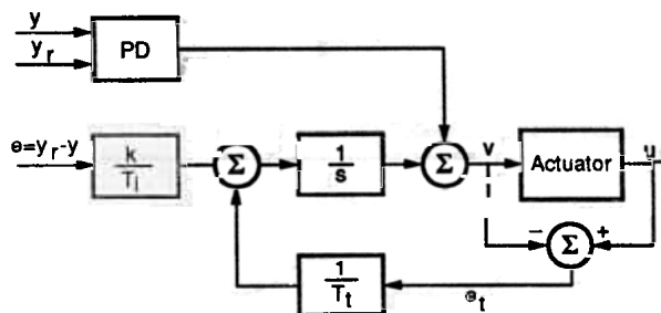
Figure 2. Regulator with anti-windup based on back-calculation.
