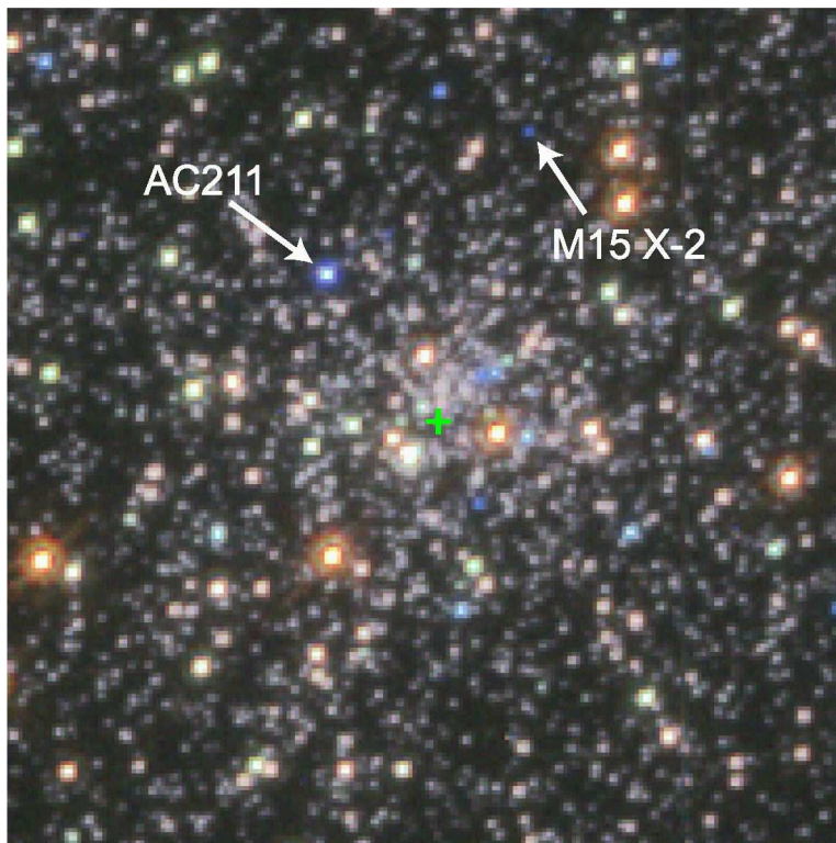
Fig. 1c.— A true color (U+B+V) Hubble Space Telescope image of the central 9''x9'' region of M15 reproduced from Guhathakurta et al. (1996). The positions of AC211 and the \sim 19^{th} U magnitude blue star identified with M15-X2 are indicated. The green cross shows the center of M15 (Guhathakurta et al. 1996). Note the orientation is different from Fig 1b.
