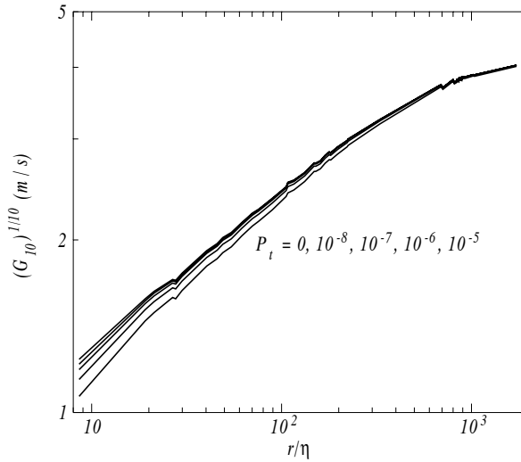
Fig. 3.11: Structure function of order 10 computed over truncated PDFs. The total probability in the discarded tails is P_t . P_t ranges from 0 (topmost curve) to 10^{-5} (lowest curve).
