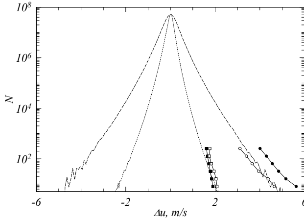
Fig. 3.24: Dependence of the amplitude of mean worms, found at separations r/\eta \sim 9 , on the length of the search list N . The results ( \bullet, \circ original data, \blacksquare, \square scrambled data; filled, empty markers: transverse, respectively longitudinal worms) are compared to the corresponding probability distribution functions of velocity increments \mathcal{P}_{r/\eta}^{T,L}(\Delta u) (long-, respectively short-dash lines).
